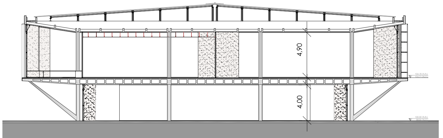
CORTE CC (TRANVERSAL) CROSS SECTION CC
