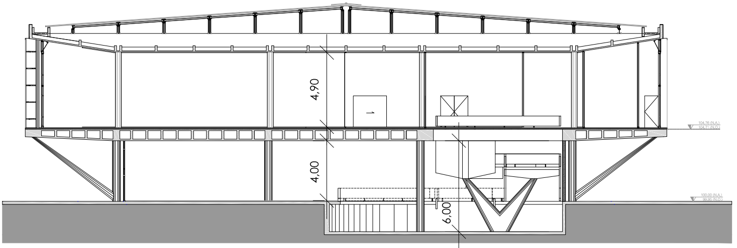
CORTE BB (TRANVERSAL) CROSS SECTION BB
